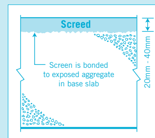
Bonded Screed
