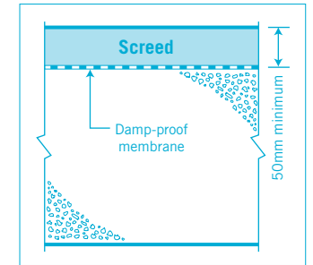
Unbonded Screed
